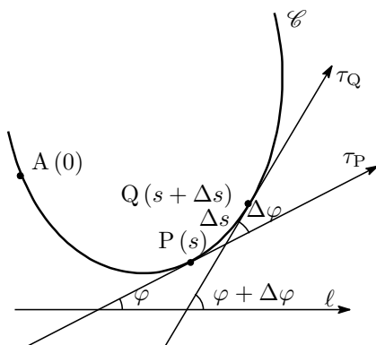
Figure 1.3: 有向接線と曲率
