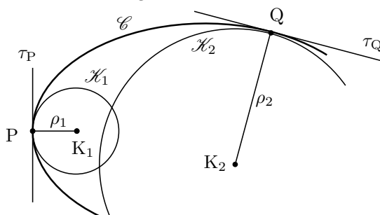
Figure 1.7: 曲率円
