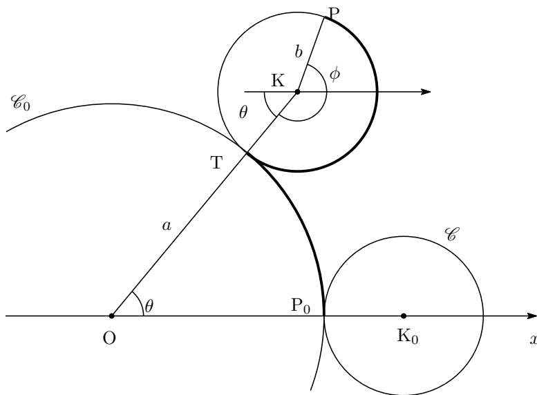
Figure 2.3: epicycloid
